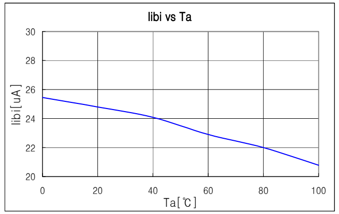
Fig. 4 Ictrl pin input bias current vs Ambient Temperature
