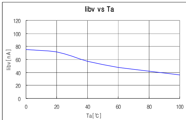
Fig. 3 Vesense pin input bias current vs Ambient Temperature
