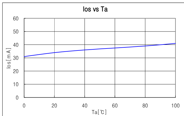
Fig.5 Output Short circuit current vs Ambient Temperature
