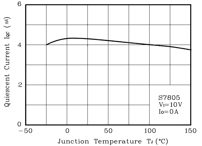
Fig. 4 I_{QC} vs. T_J
