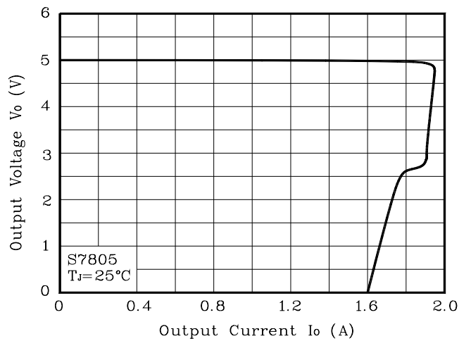
Fig. 6 V_O vs. I_O
