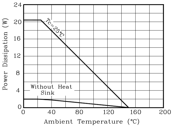
Fig. 9 P D vs. T a
