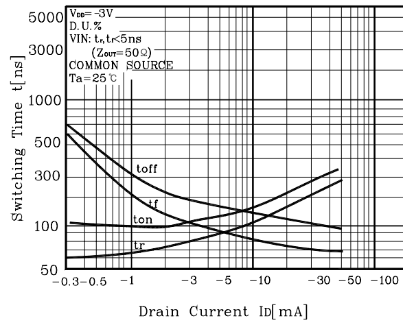
Fig8 t - Id
